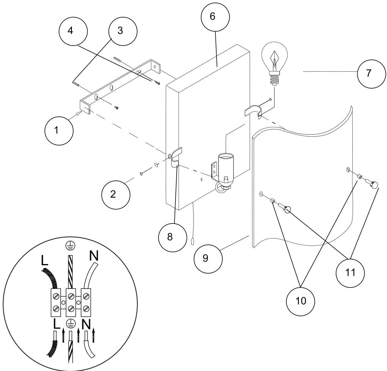
6. Details of terminal wiring.
