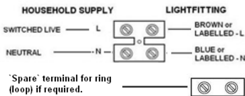
④ Details of terminal wiring.
