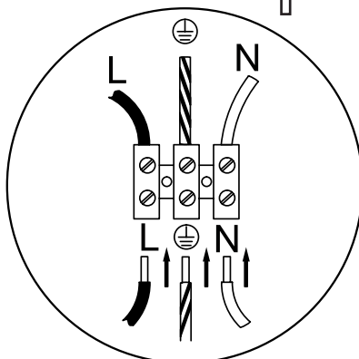
Expanded Wiring Diagram
