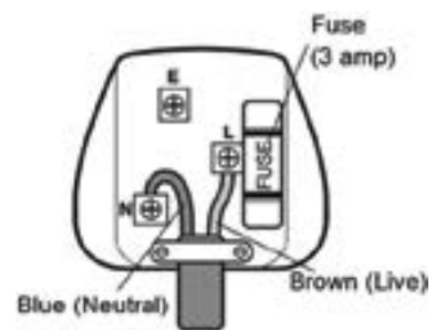
Class II Plug Wiring Diagram
