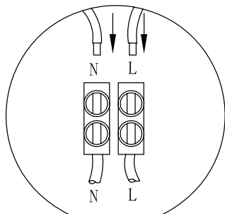
2. Expanded wiring diagram
