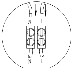
2. Expanded wiring diagram
