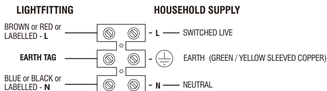
Wiring Details
