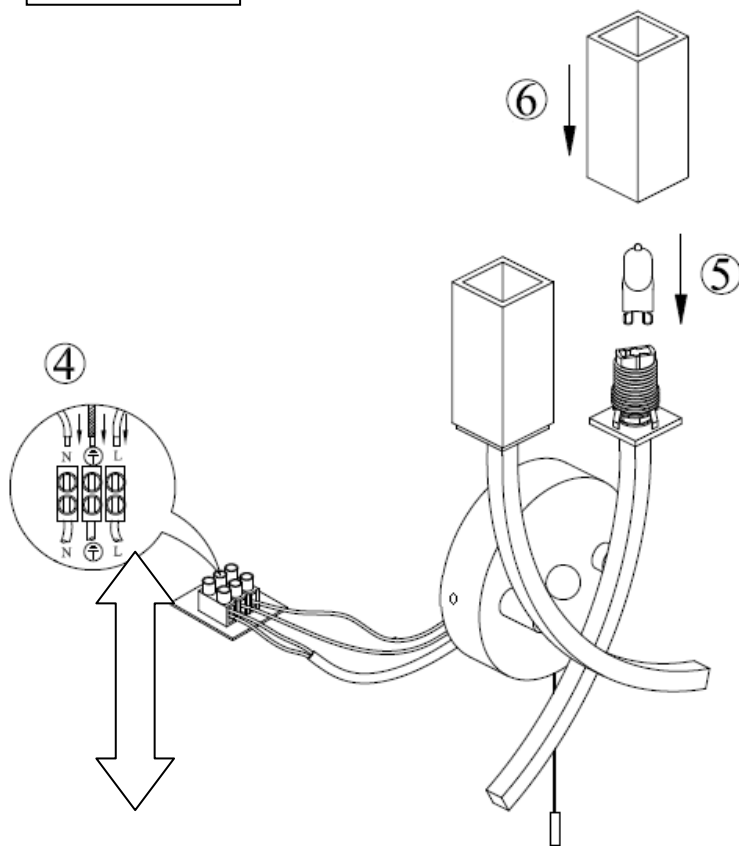
Wiring Details
