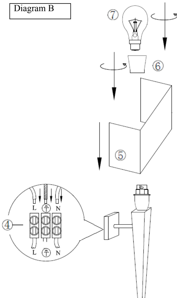
Details of terminal wiring.
