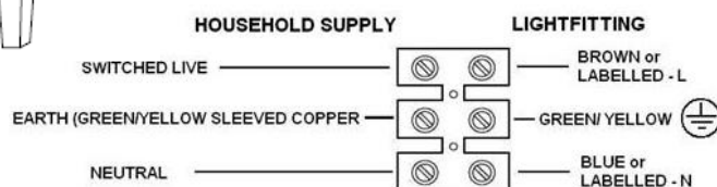
Details of terminal wiring.
