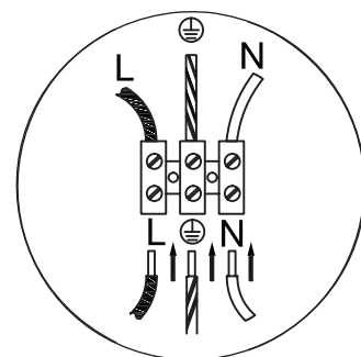
Details of terminal wiring.
